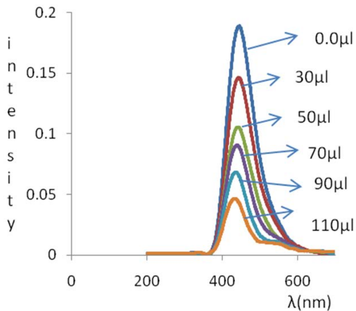
Fig.4. The changing fluorescence emission spectra of quinine ( 10^{-3} \text{ M} ) in aqueous solution with addition of 0.0, 30, 50, 70, 90, 110 \mu\text{l} \text{MnO}_4^- ( 10^{-1} \text{ M} ).
