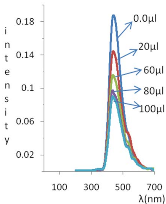
Fig. 3. The changing fluorescence emission spectra of quinine ( 10^{-3}\text{M} ) in aqueous solution with addition of 0.0, 20, 60, 80, 100 \mu\text{l} \text{Cl}^{-} ( 10^{-1}\text{M} ).
